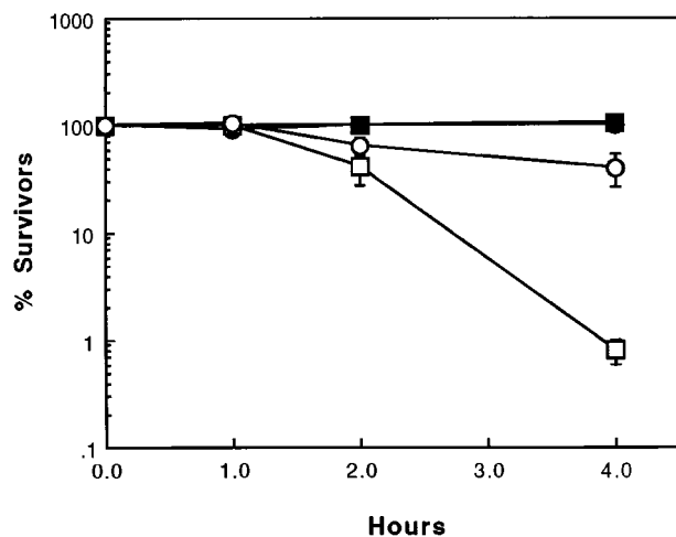
FIG. 2. Linolenic acid-sensitive phenotype of Q-deficient yeast can be rescued by the COQ3 gene on a single copy plasmid. Yeast strains FW103:pRS313 (Coq - ) (□, ■) and FW103:pCC-COQ3 (Coq + ) (○, ●) were incubated in the presence of 820 \mu M oleic (●, ■) or linolenic (○, □) acid and atmospheric oxygen as described in Fig. 1. Values are expressed as mean \pm SD of three independent experiments.
