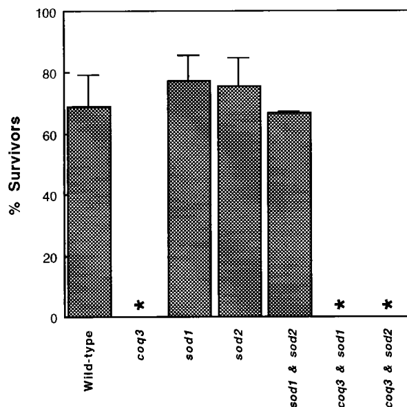
FIG. 5. Sensitivity of wild-type, Q-deficient and SOD-deficient yeast to linolenic acid. Yeast strains EG103 (wild-type), FW103 ( coq3Δ ), EG118 ( sod1Δ ), EG110 ( sod2Δ ), EG133 ( sod1Δ, sod2Δ ), CC2039 ( coq3Δ, sod1Δ ), and FW110 ( coq3Δ, sod2Δ ) were incubated with 82 \mu M linolenic acid as described in Fig. 1. Percent survivors determined after 4 h of incubation are as indicated or are less than 1% (asterisk). Values are expressed as mean \pm SD of two measurements.
